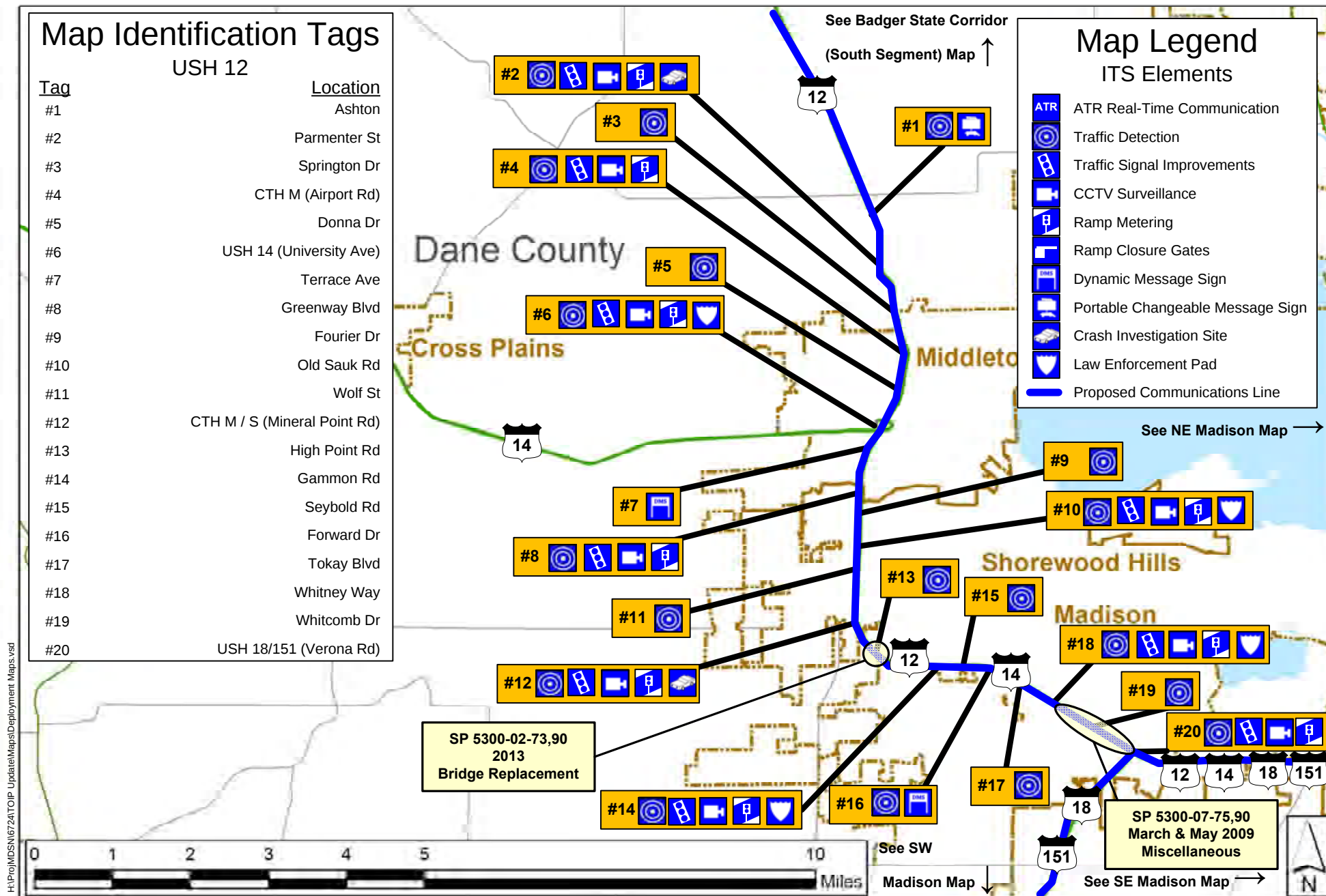
Northwest Madison – TOIP Based ITS Deployment
